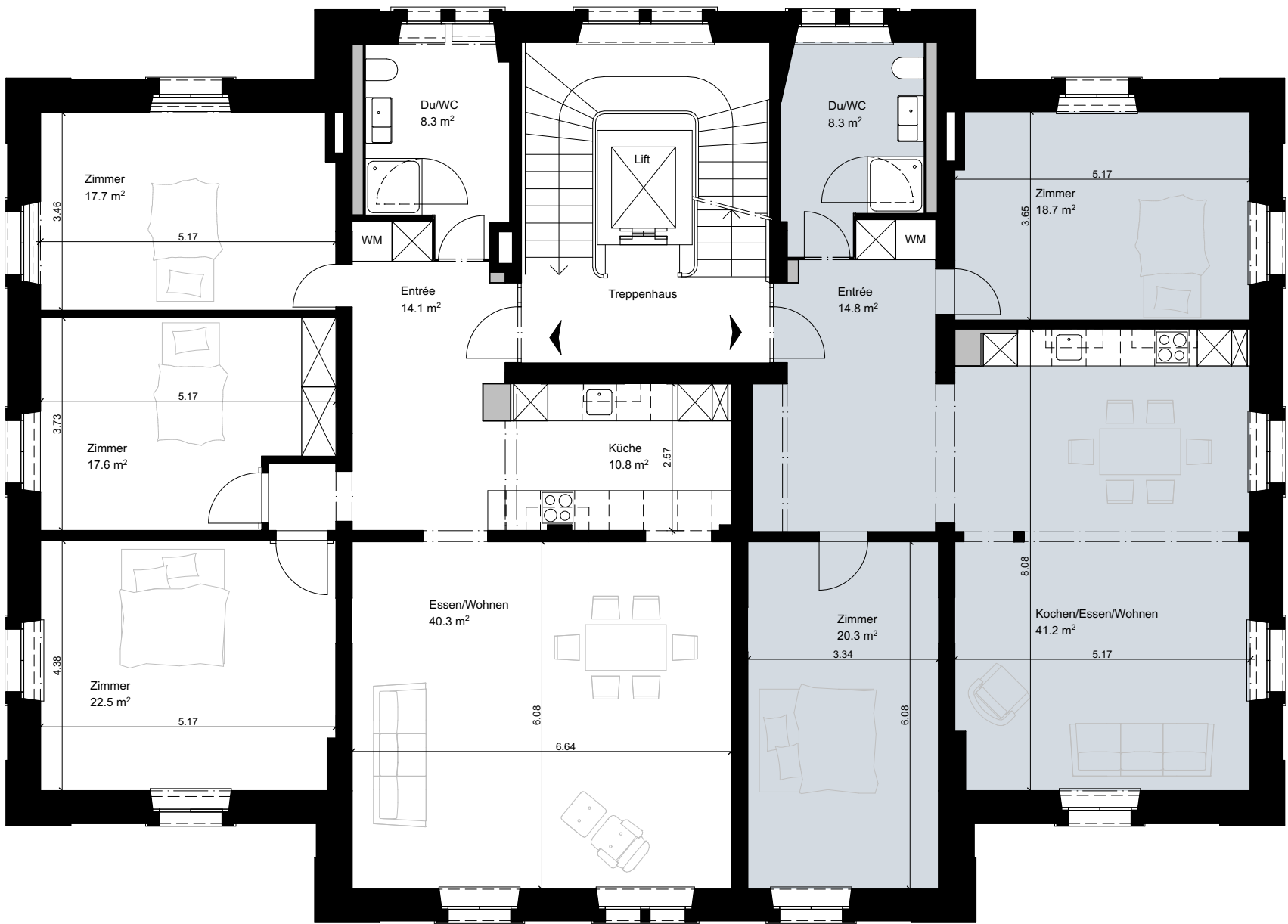
2.OG West - 4½ Zi-Whg NTWF: 131.2 m²
