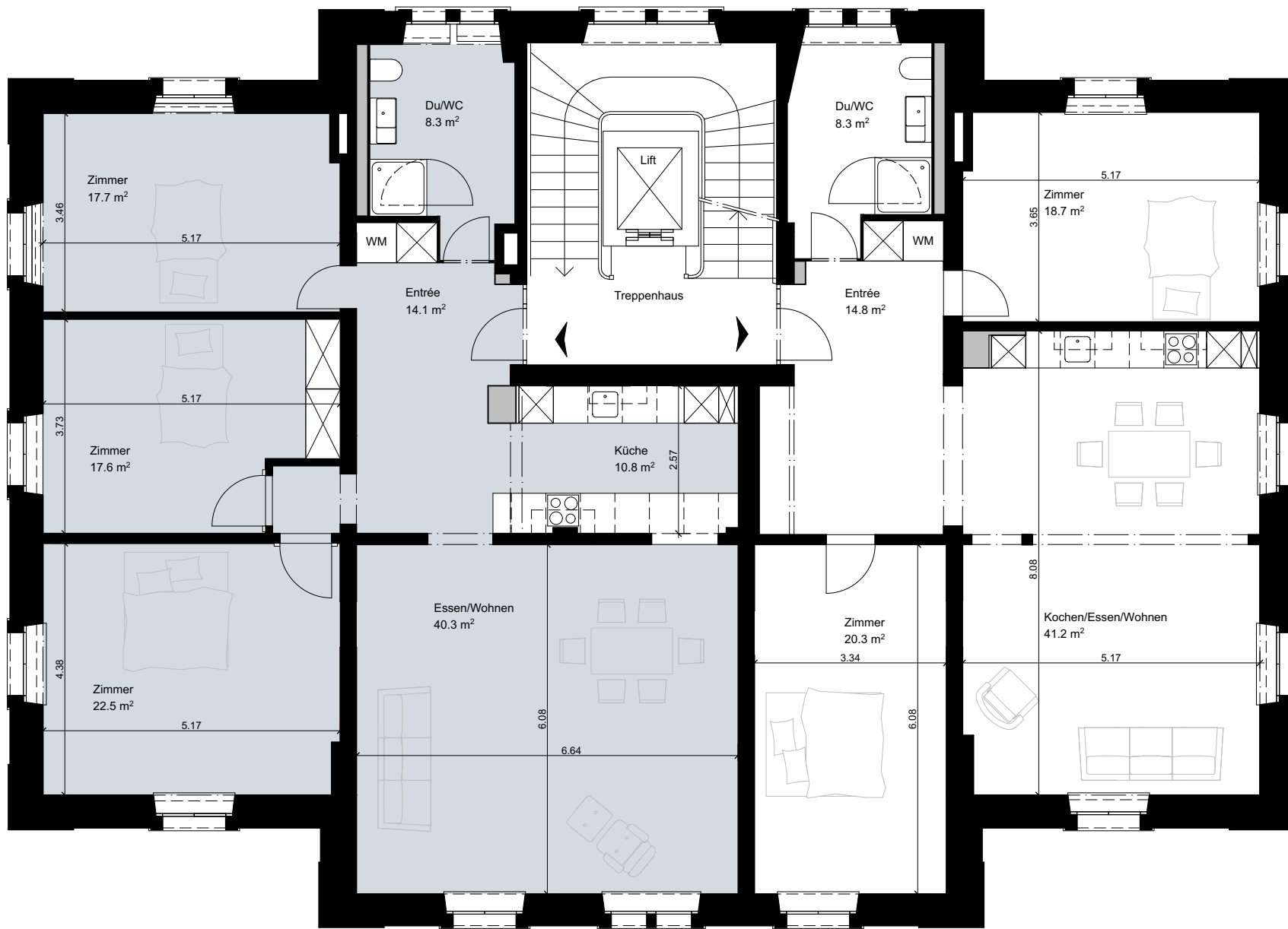
2.OG Ost - 3½ Zi-Whg NTWF: 103.3 m²
